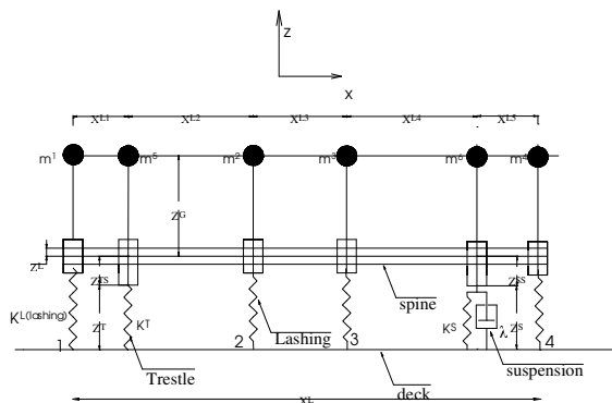
Fig. 5: Simplified model of the trailer
