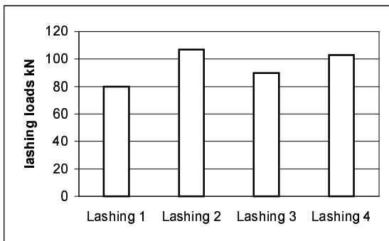
Fig. 15: Maximum loads on each lashing for the parameter values shown in Table 5.
